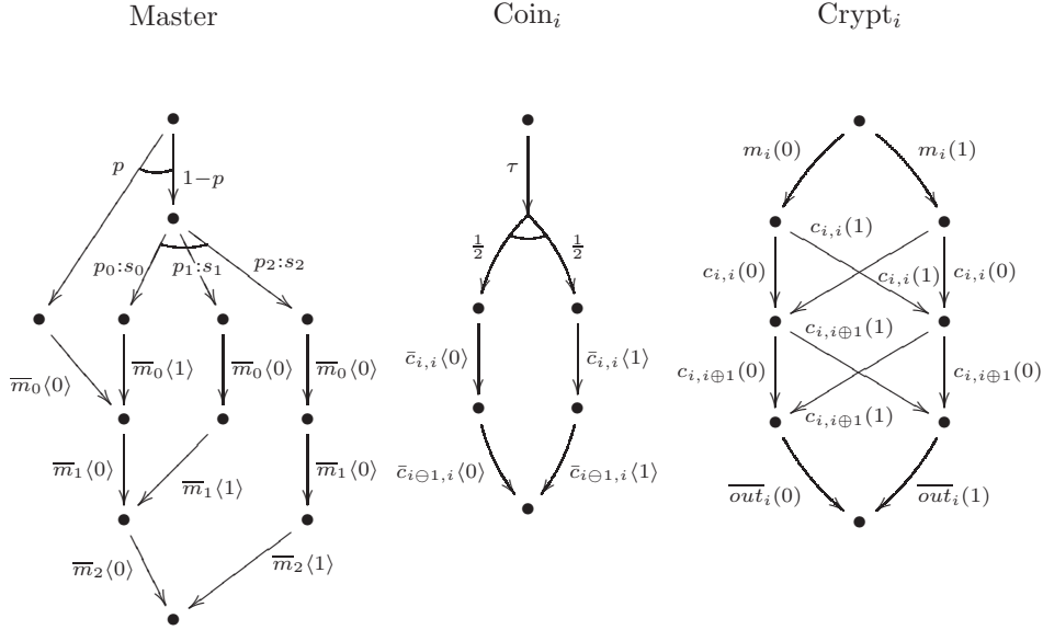
Figure 3: Dining Cryptographers Automata
