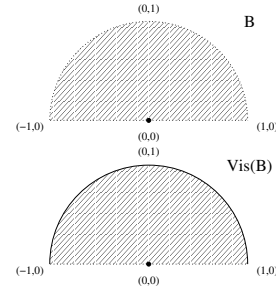
Figure 2 B and \text{Vis}(B)
