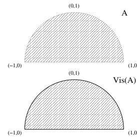
■ Figure 1 A and \text{Vis}(A)
