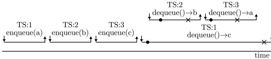
Figure 1: Example where the optimization is fair but unsound according to linearizability.
